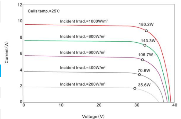
I-V Curves at different irradiance
